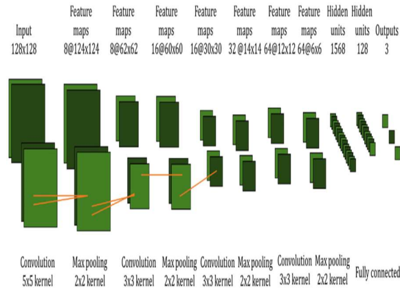
Fig.5.Proposed Deep CNN Model
