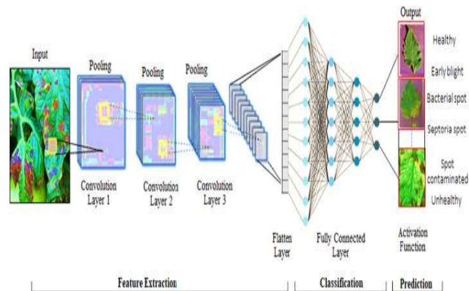
Fig.1 Architecture of CNN
