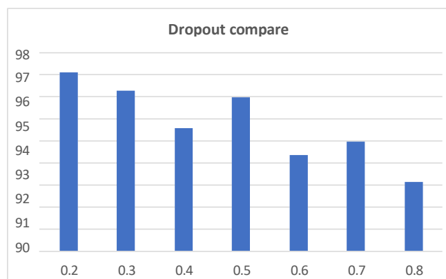
Fig.6.Validation accuracy for various dropouts
