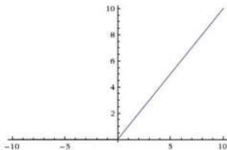
Fig.2.ReLuActivationFuinction
