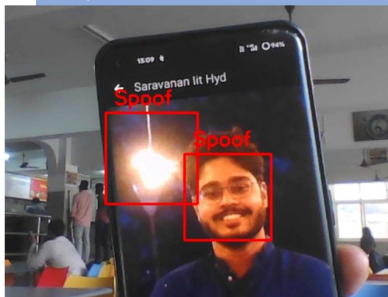
Fig 2: Spoof detection
