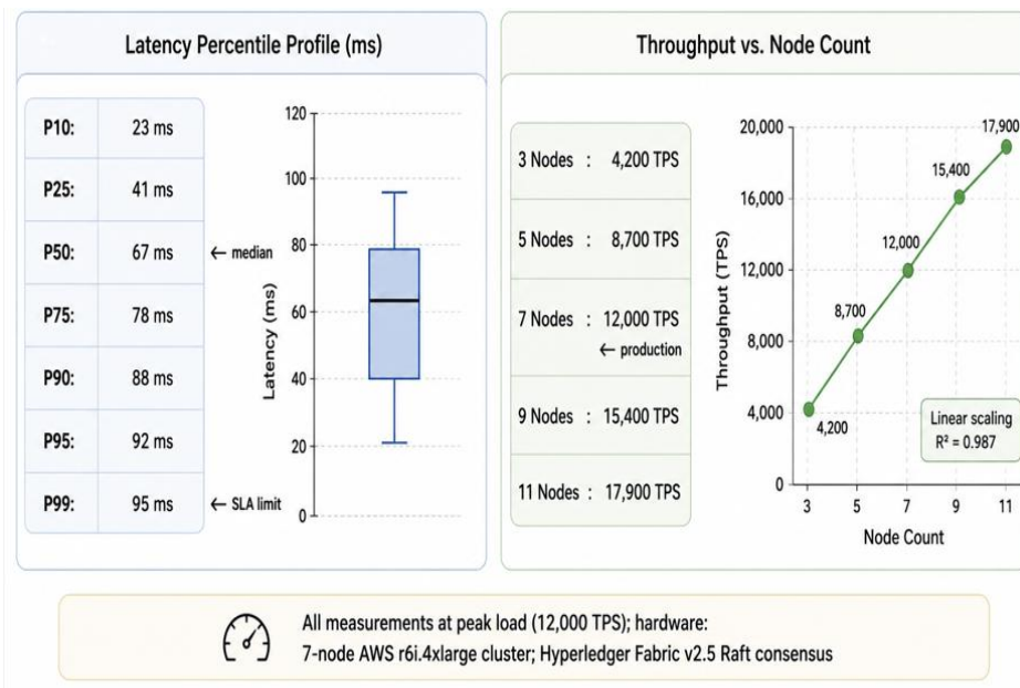
Figure 2. Latency percentile profile (left) and horizontal throughput scaling (right) .
