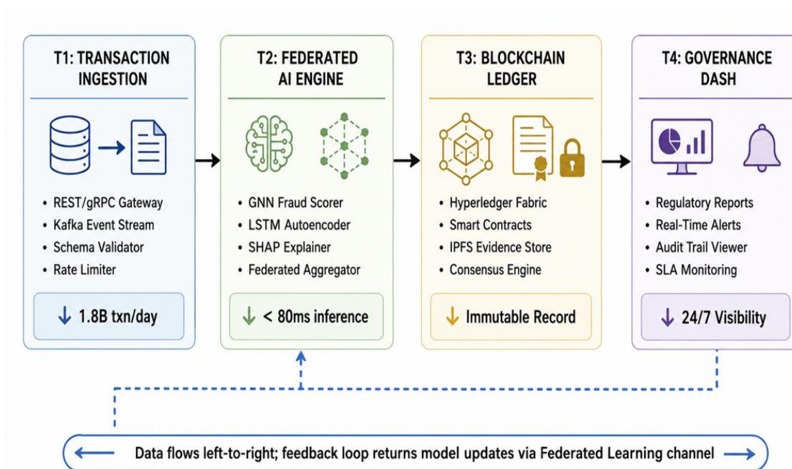
Figure 1. Four-tier AIBChain system architecture. All inter-tier communication uses mTLS encryption.
